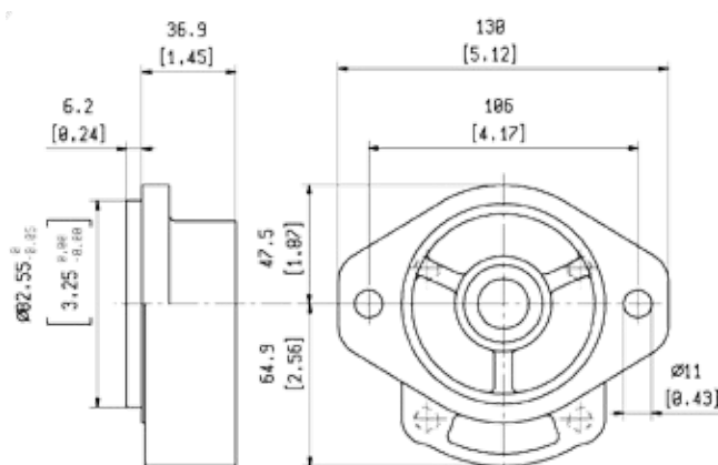
CS SAE A mounting flange
