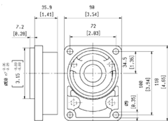
CB German standard mounting flange
