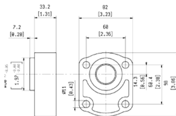
CL For engine endo thermic motors mounting flange
