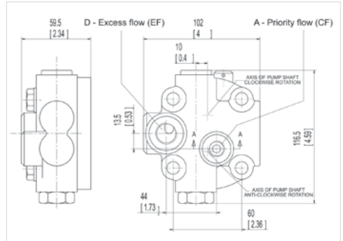
VP - VPS REAR PORTS
