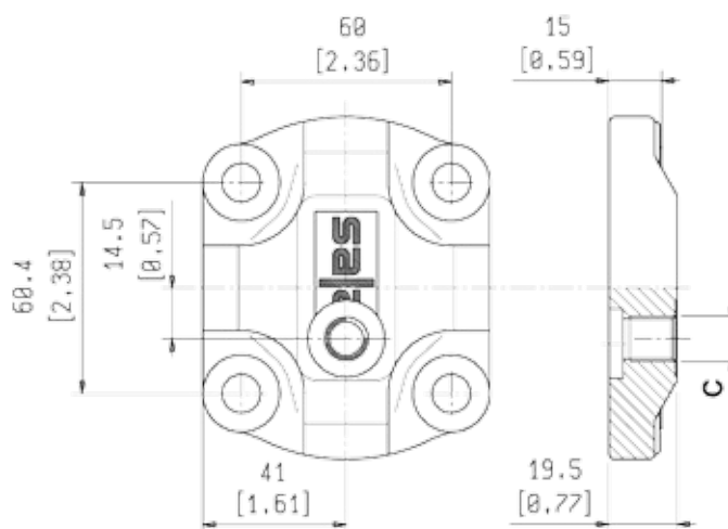
Standard rear cover for reversible pumps and motors, with external drain \Phi C . For the dimension \Phi C please see the table here below
