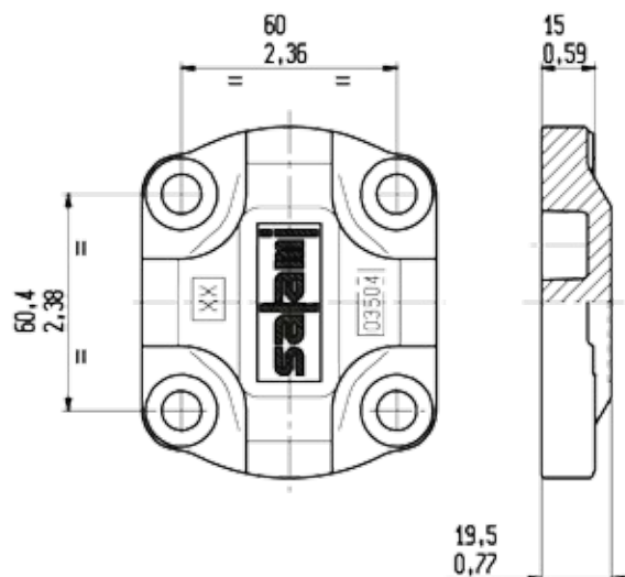
Standard rear cover for unidirectional pumps and motors
