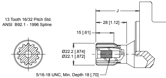
01 7/8" 13 Tooth Spline
