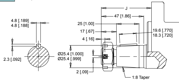
13 1" Tapered
