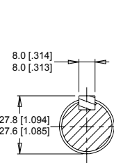
12 25mm Straight
