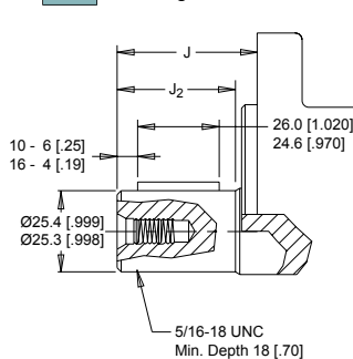
15 1" Straight Extended
