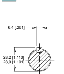
10 1" Straight
