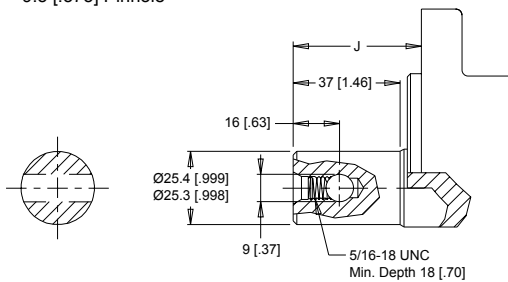
05 1" - 9.5 [.375] Pinhole
