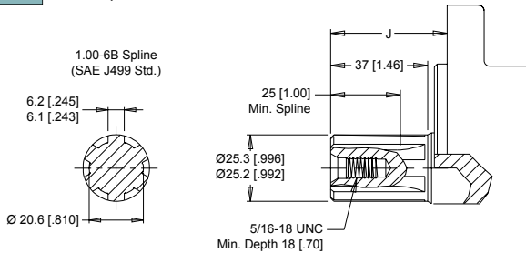
02 1" 6B Spline
