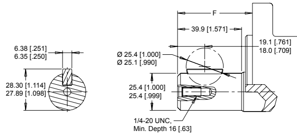
B1 1" Straight, Woodruff Key
