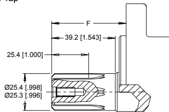
04 1" 6B Spline, M8x1.25 Tap
