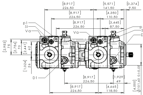
Shafts for combination pumps
