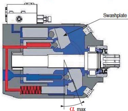
Figure 1 - Maximum displacement
