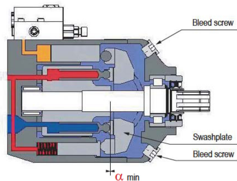
Figure 2 - Zero displacement
