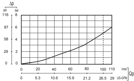
Main anticavitation valve curve
