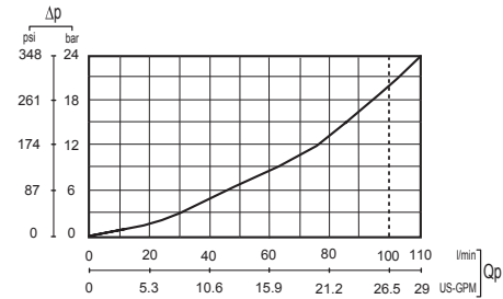
Anticavitation check valve curve
