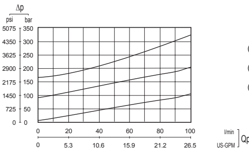
Hydraulic pilot control curve
