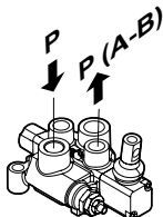
Pressure drop with spool in working position
